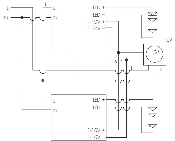
1-10V Connections
