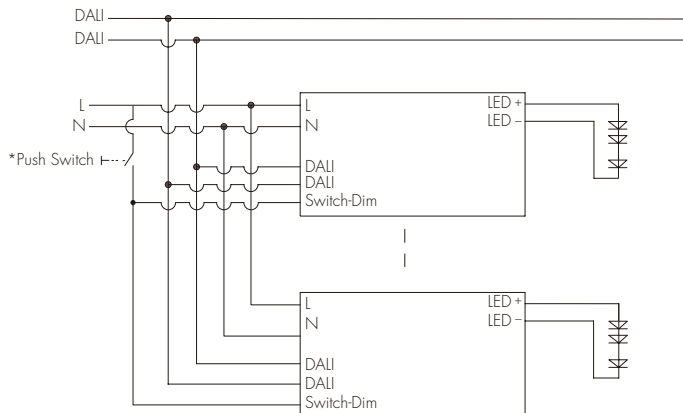
DALI Connections
